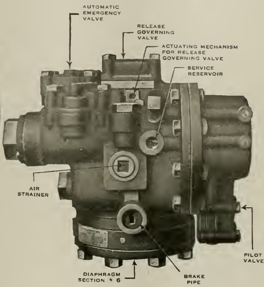
TYPE S-2 FRONT VIEW. TRIPLE VALVE
